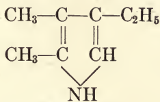
Ischæmopyrrol β-ethyl, α'-β'-dimethyl pyrrol
